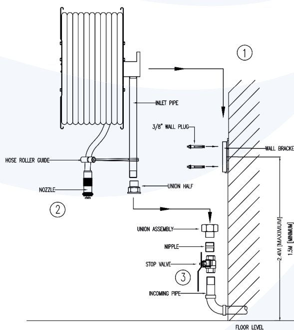
Fixed Hose Reel
