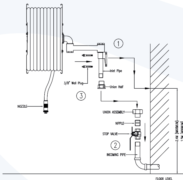
Swinging Hose Reel
